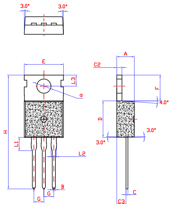
TO-220C
