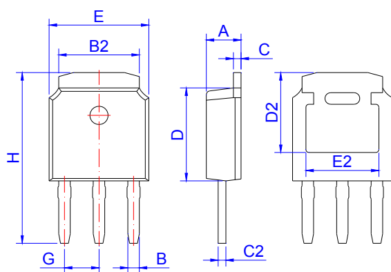
TO-251-4R
