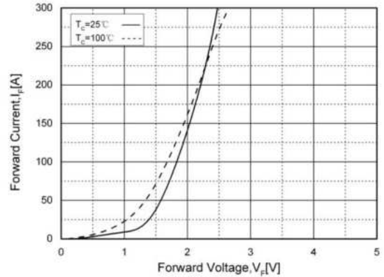
Fig. 10. Forward Characteristics
