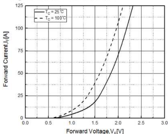
Fig. 10. Forward Characteristics
