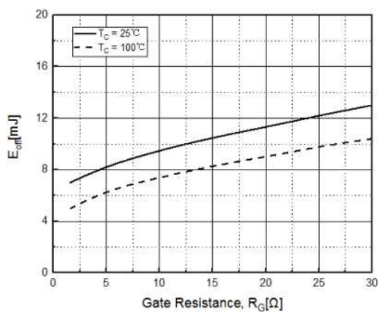
Fig. 6. Turn-off Characteristics vs. R_G
