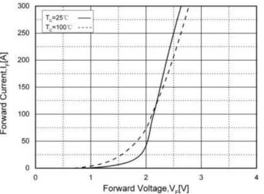
Fig. 10. Forward Characteristics
