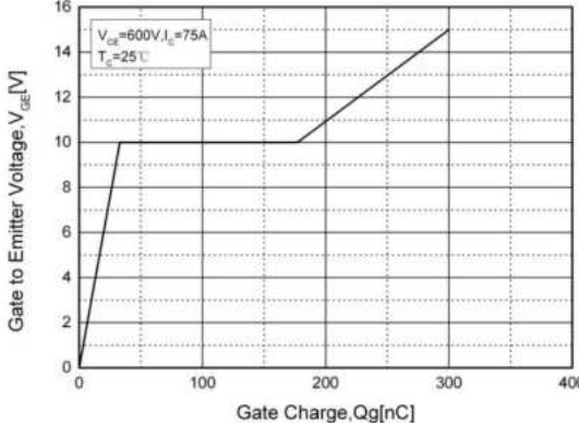
Fig. 4. Gate Charge Characteristics
