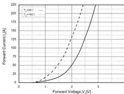
Fig. 10. Forward Characteristics
