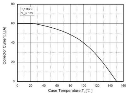
Fig. 7. Rate Current vs. T_C
