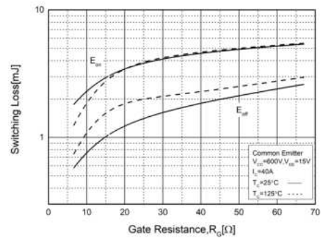
Fig. 8. Switching Loss vs. R_G
