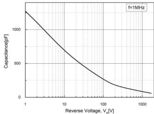
Fig. 4. Typical Characteristics: V_R vs. Capacitance
