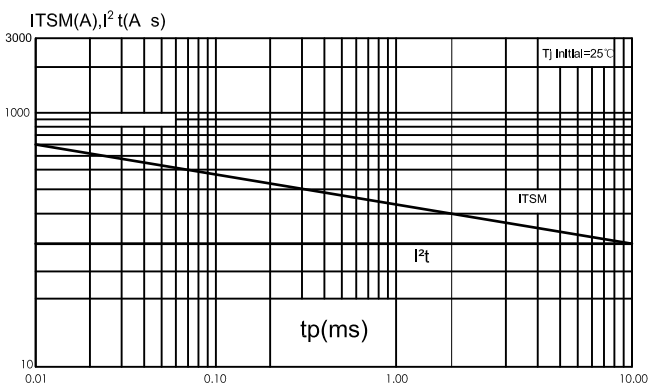
Fig.5 : Non-repetitive surge peak on-state current for a sinusoidal pulse with width t_p < 20\text{ms} and corresponding value of I_t t ( dI/dt < 100\text{A}/\mu\text{s} )
