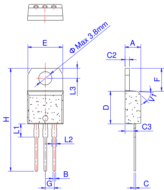
TO-220A/B
